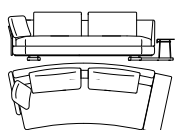
822-25-FS_L04_R07 B 287 T 121 H 85/87 SH 43/45 ST 60 AH 60/62
