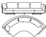
822-30-FS_L04_R04 B 299 T 150 H 85/87 SH 43/45 ST 60 AH 60/62
