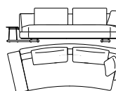
822-25-FS_L07_R04 B 287 T 121 H 85/87 SH 43/45 ST 60 AH 60/62
