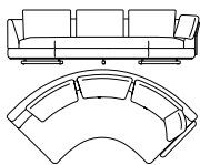
822-30-ES_L00_R04 B 296 T 150 H 85/87 SH 43/45 ST 60 AH 60/62
