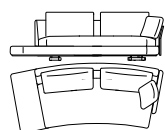
822-20-FS_L01_R04 B 274 T 121 H 85/87 SH 43/45 ST 60 AH 60/62
