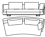
822-25-AS_L00_R04 B 254 T 120 H 85/87 SH 43/45 ST 60 AH 60/62
