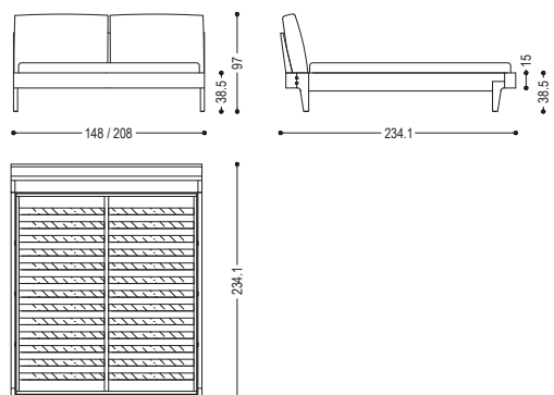
REVO BED SOFT DOUBLE - REVO BED SOFT FRENCH
