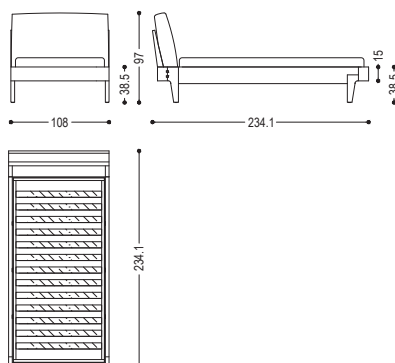
REVO BED SINGLE
