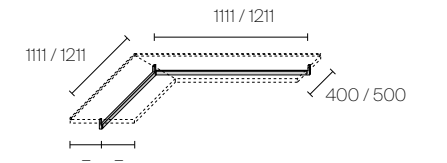
Clothes-hanger for corner shelf or top
