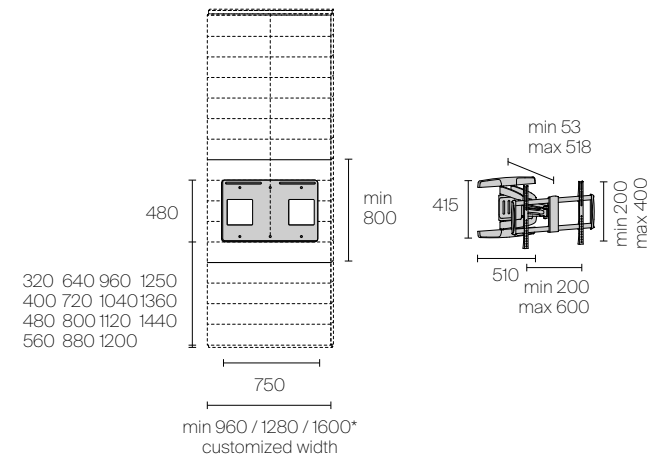
Version in saharah wood, taiga wood, fabric, synthetic leather available only in W 960 / 1280 *W 1600 available only for equipped open unit
