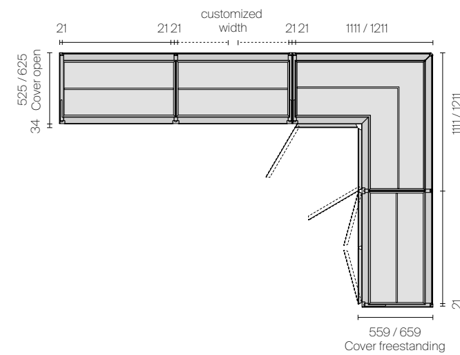
Corner composition Cover Open + Cover freestanding
