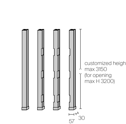
Structural upright
