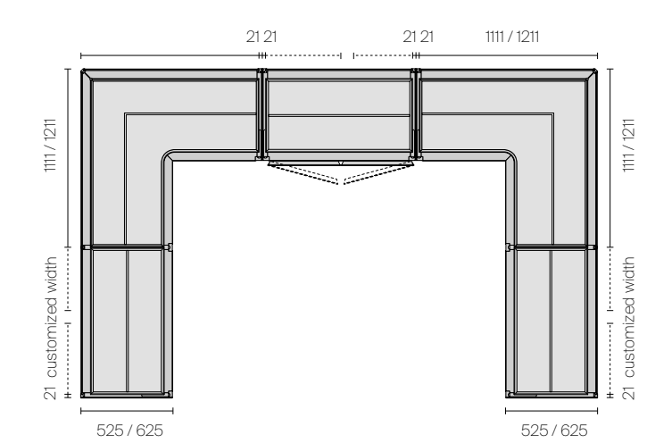
C-shaped composition Cover Open + Cover freestanding
