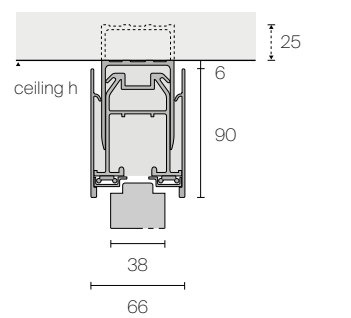
Double rail
