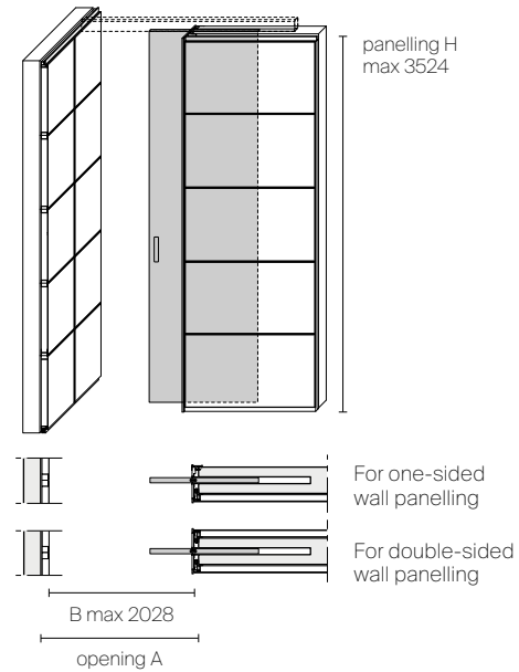
Full-height single pocket door against Modolor panel
